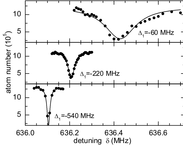
Figure 6.5: Two-color photoassociation spectra of the second to last bound state in the ^{87}\text{Rb } a^3\Sigma_u^+ potential, called state |2\rangle . Shown are scans of the detuning \delta of the second laser from laser 1. The lines are Lorentzian fits to determine resonance positions and widths. For these data the intensities of both lasers are set to about 3\text{ mW/cm}^2 . From top to bottom, the detuning of laser 1 from the intermediate state |1\rangle = |O_g^-(\sim S_{1/2} + P_{1/2}), v = 21, J = 0\rangle is set to \Delta_1 = -60\text{ MHz} , -220\text{ MHz} and -540\text{ MHz} .
