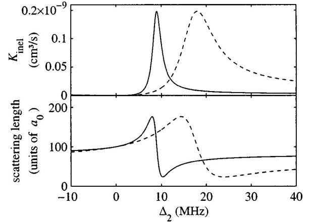
FIG. 2. K_{\text{inel}} and scattering length a according to Eqs. (1) and (2), plotted for two values of \Delta_1 . Solid line: \Delta_1/2\pi = 100 MHz. Dashed line: \Delta_1/2\pi = 50 MHz. The other parameters are \Gamma_{01}/2\pi = 50 kHz, \Omega_{12}/2\pi = 30 MHz, and \gamma_1/2\pi = 25 MHz. The wave number k_i = 2.5 \times 10^5 \text{ m}^{-1} corresponds to the finite size of the condensate wave function. a_0 is the Bohr radius.
