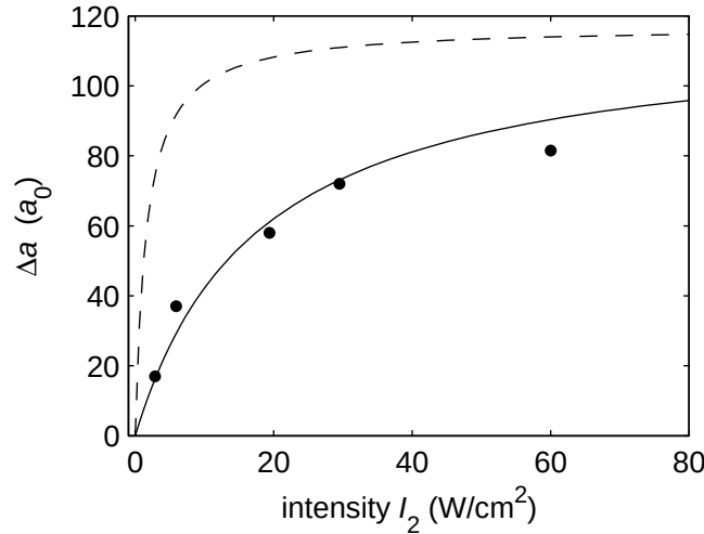
Figure 6.15: Maximum tuning range \Delta a of the scattering length versus intensity I_2 . The experimental data are obtained for \Delta_1/2\pi = 60 \text{ MHz} and an intensity I_1 = 300 \text{ W/cm}^2 . For every data point a full resonance curve is taken, from which we determine \Delta a = a_{\text{max}} - a_{\text{min}} . The figure also displays the results of our extended theoretical model (see section 6.4.3). While for the dashed line \gamma_2/2\pi is set to 100 \text{ kHz} , the solid line corresponds to \gamma_2/2\pi = 2 \text{ MHz} .
