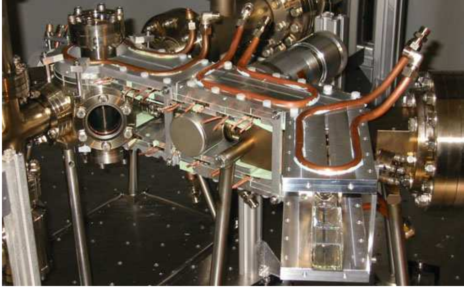
Figure 4.8: Magnetic coils and cooling bars of the transfer line. In this photo the last transfer section is not mounted except for the cooling bars above and below the glass cell.
