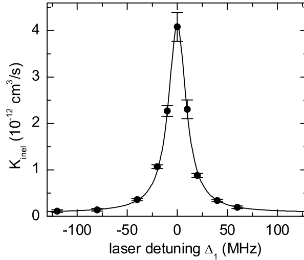
Figure 6.2: Losses from a BEC due to photoassociation. The inelastic collision rate coefficient K_{\text{inel}} is plotted for a coupling to the molecular state |O_g^-(\sim S_{1/2} + P_{3/2}), v=1, J=2\rangle . Here the laser intensity is 20 \text{ W/cm}^2 and the peak density 3.3 \times 10^{14} \text{ 1/cm}^3 . From a Lorentzian fit to the data (solid line) we derive the parameters \gamma_1 = 21 \text{ MHz} and \Gamma_{\text{stim}} = 2.4 \text{ kHz} . To quote a value for \Gamma_{\text{stim}} , a collisional wave vector of k = 2.47 \times 10^5 \text{ m}^{-1} is used.
