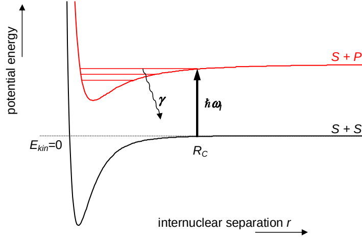
Figure 2.5: Schematic diagram of the molecular potential for two ground-state atoms ( S + S ) and an attractive excited potential connecting to an S + P asymptote. An optical free-bound transition and the subsequent decay are indicated.
