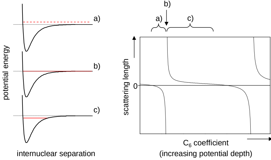
Figure 2.3: Dependence of the scattering length on the position of the last bound state. Increasing the potential depth, e.g. by increasing the C_6 coefficient, results in a divergence of a whenever a new bound state appears: A virtual bound state close above threshold corresponds to a negative scattering length a), which diverges if a real bound state appears b), and becomes positive for a weakly bound state just below threshold c).
