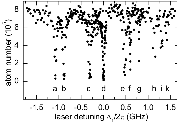
Figure 6.1: Photoassociation spectrum of the |1_g(\sim S_{1/2} + P_{3/2}), v = 152\rangle state. The atom-loss spectrum is obtained after illuminating a BEC for 5 \text{ ms} with a laser intensity of 90 \text{ W/cm}^2 . In the plot we have arbitrarily chosen the zero of the detuning to coincide with the line labelled d. We can assign the lines a to k to molecular quantum numbers by comparing the measured spectrum to a calculation by E. Tiesinga [Tie04b]. The lines share the same total nuclear spin i = 3 , but have different values \iota for the projections of i onto the molecular axis. As \iota is almost a good quantum number, it has fractional values close to integers. Further, the states depend on the total angular momentum f . We assign the following quantum numbers (f, \iota) to the lines: a \leftrightarrow (2, -2.971) , b \leftrightarrow (3, -2.929) , c \leftrightarrow (1, -1.97) and (2, -1.94) : not resolved, d \leftrightarrow (3, -1.895) , e \leftrightarrow (1, -0.982) , f \leftrightarrow (2, -0.948) , g \leftrightarrow (3, -0.9) , h \leftrightarrow (1, -0.048) , i \leftrightarrow (2, -0.005) , k \leftrightarrow (3, 0.053) .
