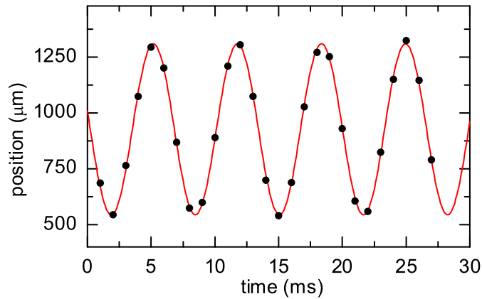
Figure 5.3: Trap frequency in radial direction for ^{87}\text{Rb} |F = 1, m_F = -1\rangle atoms in the QUIC trap at a current of 40 A. The measured oscillation of the atoms in the trap is shown together with a sine-curve fitted to the data.
