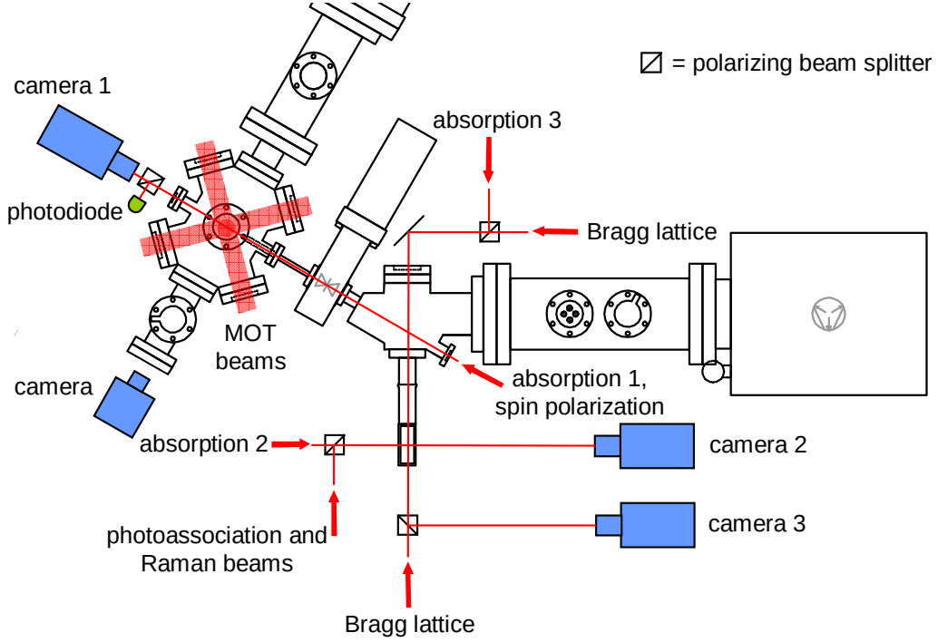
Figure 4.13: Arrangement of the laser beams and imaging system. The figure shows the installed cameras together with the paths and directions of the most important laser beams. The numbers of the cameras can be used to identify the corresponding absorption beams. Information on the Bragg lattice laser beams also shown in this figure can be found in section 6.2.2.
