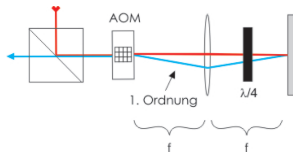
Abb. 5.1: Double-Pass-AOM Konfiguration
