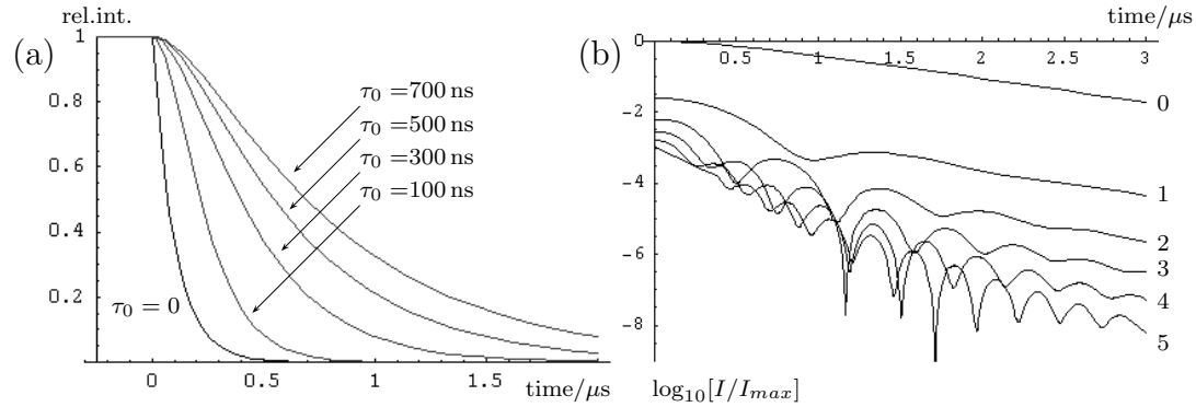
Figure 6.2: CRD with the input field switched off slowly. a) For different \tau_0 with \tau = 100 ns and \delta=0 . b) Non-resonant decay with the numbers corresponding \delta in units of \pi/1000 . \tau = 633 ns and \tau_0 = 200 ns.
