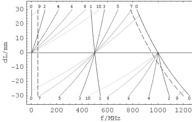
Figure 2.17: Frequencies of the first 10 transversal \text{TEM}_{mn} modes of a cavity around confocal configuration. The numbers correspond to m + n . One FSR = 1 GHz is drawn with the mirror distance is varied by dL = \pm 30 mm around L = 150 mm. r_1 = r_2 = 150 mm.
