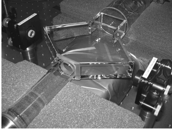
Figure 3.14: Photo of glasscell with testing resonator.
