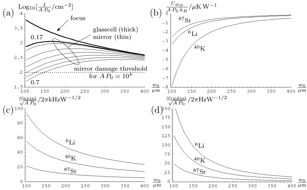
Figure 3.22: a) Intensity (logarithmic scale) in focus, on glasscell ( L=0.17 m) and on mirrors for different distances of mirrors from L=0.2 m to L=0.7 m in steps of 0.1 m. b) Trap depth, c) axial trap frequencies and d) radial trap frequencies. All normalized by total power.
