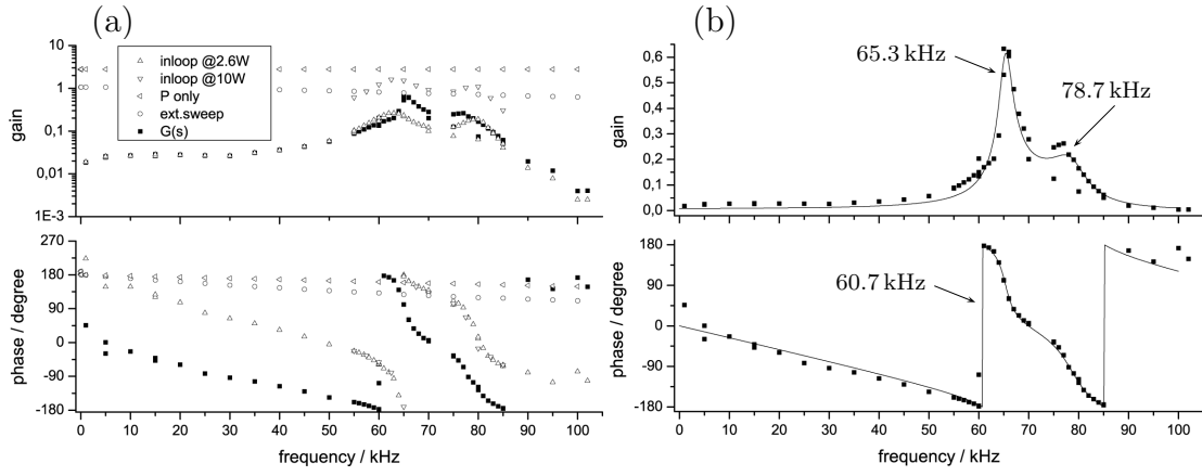
Figure 3.9: a) Measurement of the transfer function of the PDH lock of the laser. b) Fit of the transfer function gives position and width of two piezo resonances.
