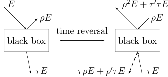
Figure 2.5: Time reversal symmetry causes a relative phase jump of \pi in reverse direction with respect to forward direction
