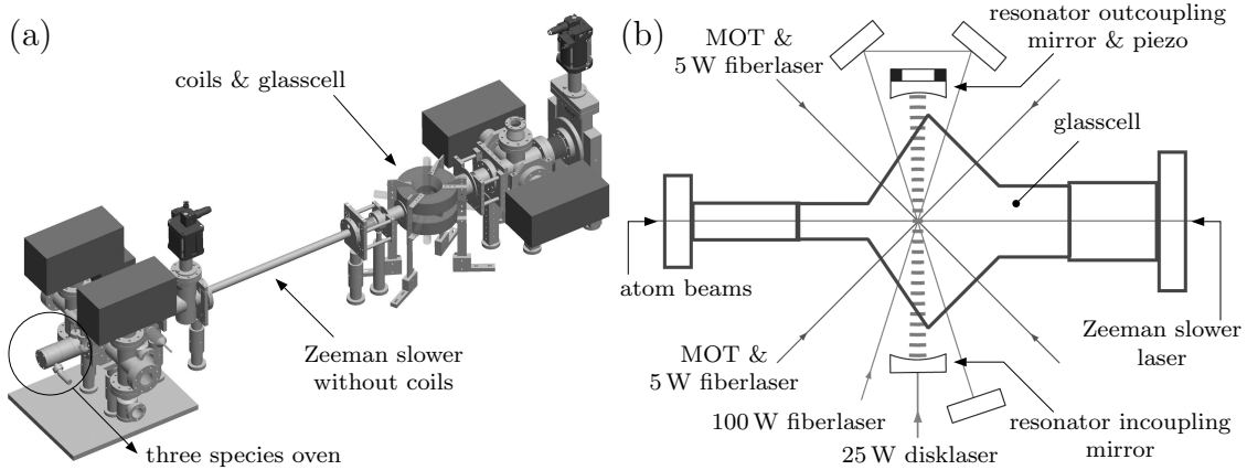
Figure 1.1: a) Experimental setup and b) glasscell with trapping laser beams.
