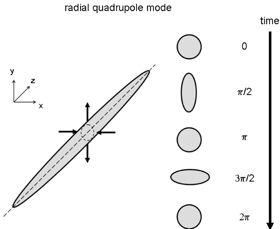
Figure 3.4: Radial quadrupole mode of an elongated cloud. The cloud is tightly confined in the radial x - and y -directions and weakly confined in the axial z -direction. The surface of this mode is oscillating and no compression takes place.
