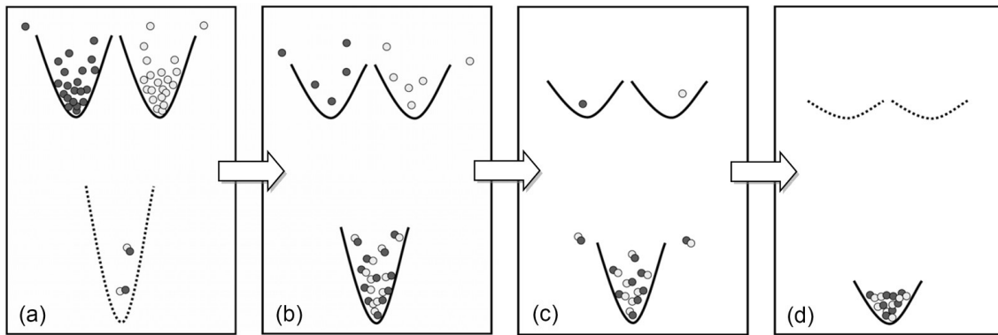
Figure 5.2: Different stages of the evaporative cooling process. (a) At high temperatures, only few molecules are present and the evaporation is mainly driven by elastic collisions in the atomic spin mixture. (b) As the gas gets colder, the chemical atom-molecule equilibrium begins to favor the molecules. (c) By further evaporation all the atoms are removed. This is further enhanced by the fact that the trap depth for the molecules is twice as large as for the atoms. Thus more molecules remain trapped. (d) After all the atoms are removed, the evaporation takes place with a purely molecular gas. Finally the critical temperature T_C is reached and the gas is condensed in a BEC.
