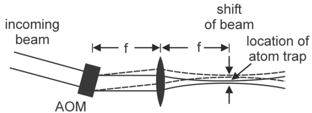
FIG. 2: Schematic illustration of the scanning system. A wide collimated beam passes through an AOM. The resulting deflection angle depends on the driving frequency of the AOM. The beam passes through a lens at the distance of one focal length behind the AOM. The lens focuses the beam for atom trapping. A change in deflection angle results in a parallel shift of the beam position in the focal plane. The solid and dashed lines show the beam path for different deflection angles. The zeroth order beam is not shown.
