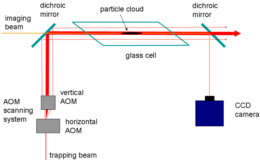
Figure 4.2: Schematic overview of the scanning system together with the imaging system along the symmetry axis of the cloud. Two crossed AOMs allow for horizontal and vertical displacement of the trapping beam. The thick solid line represents the unmodulated trapping beam. The dotted lines represent the trapping beam with maximal modulation in horizontal direction, so that the horizontal beam width is largely increased.
