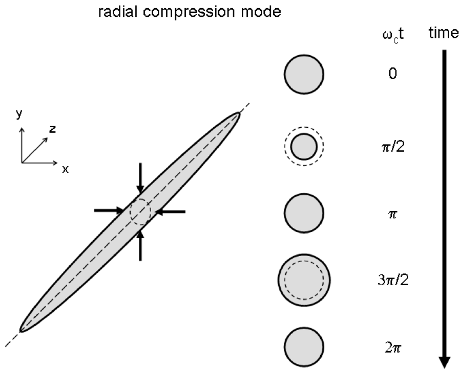
Figure 3.2: Radial compression mode of an elongated cloud. The cloud is tightly confined in the radial x - and y -directions and weakly confined in the axial z -direction. A periodic compression and decompression of the cloud along the radial directions takes place.
