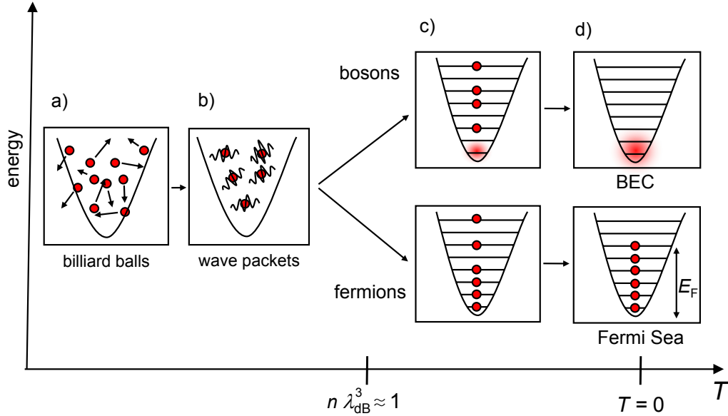
Figure 2.1: Transition from a classical gas of identical particles into a quantum mechanically governed degenerate gas. At high temperature the mean interparticle distance is much larger than the size of the particles and they can be considered as point-like (a). If the temperature is lowered, the wave-packet nature of the particles gives rise to quantum mechanical behavior (b). For temperatures where the de Broglie wavelength is on the order of the interparticle spacing ( n\lambda_{\text{dB}}^3 \approx 1 ), bosons begin to form a BEC and occupy the ground state of the trap (c, upper row). fermions however fill up the lowest lying states, occupying each state by only one particle (c, lower row). In the limit of T = 0 a pure BEC and a completely filled Fermi sea are formed, respectively (d).
