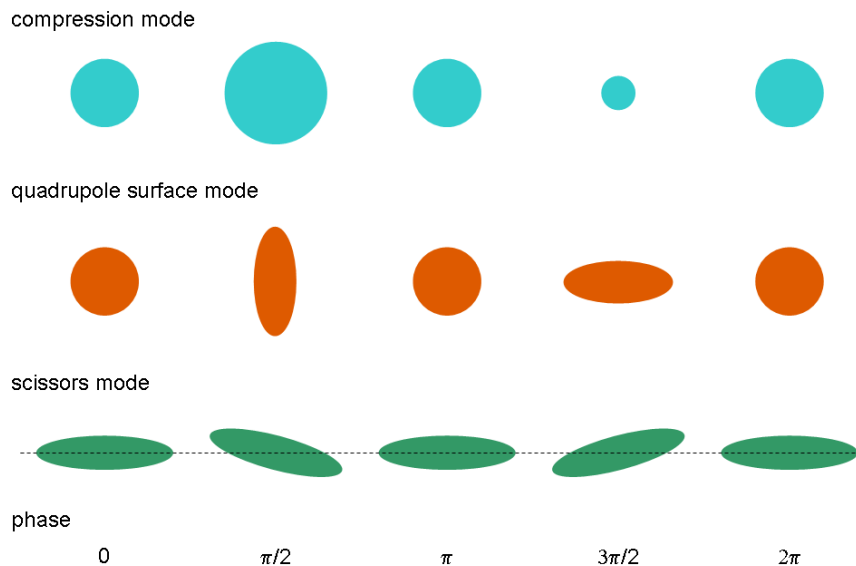
Figure 3.1: Scheme of the different radial collective oscillation modes described in this chapter: Compression mode (upper row), quadrupole surface mode (middle row) and scissors mode (lower row).
