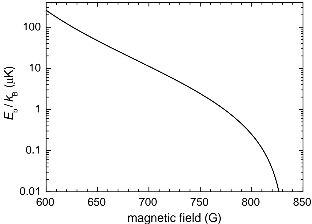
Figure 2.5: Calculated molecular binding energy for {}^6\text{Li} molecules. The calculation is based on equation 2.36. The units are chosen for comparison with experimental temperatures ( k_B \times 1\mu\text{K} \approx h \times 20.8\text{kHz} ).
